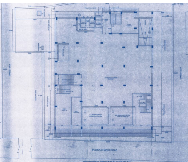
PROPOSED GROUND FLOOR PLAN SCALE: 1:100
