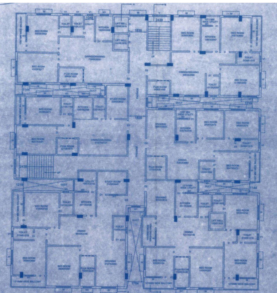
PROPOSED 3RD. FLOOR PLAN SCALE-1:100
