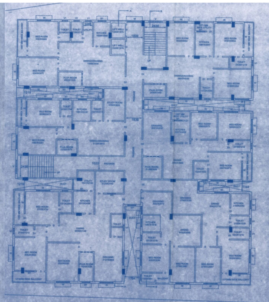
PROPOSED 4TH., 5TH. & 6TH. FLOOR PLAN SCALE-1:100
