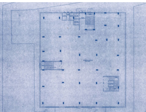
PROPOSED 2ND FLOOR PLAN SCALE: 1:100
